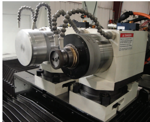
Two GMN 150mm 24,000 RPM spindles with diamond grinding wheels
