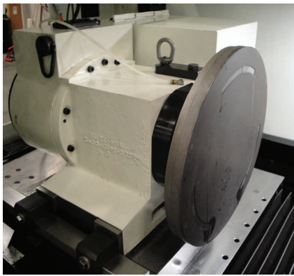
Heavy-duty workhead with custom vacuum chuck assembly
